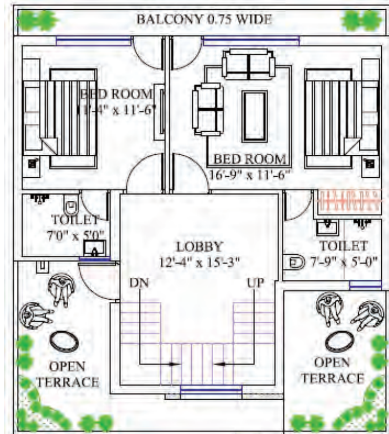
FIRST FLOOR AREA
