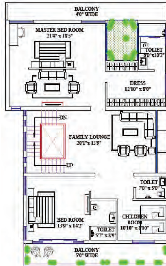
FIRST FLOOR AREA
