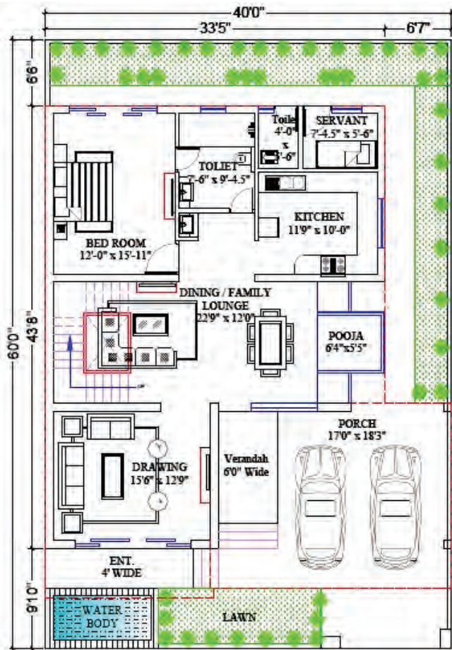
GROUND FLOOR AREA
