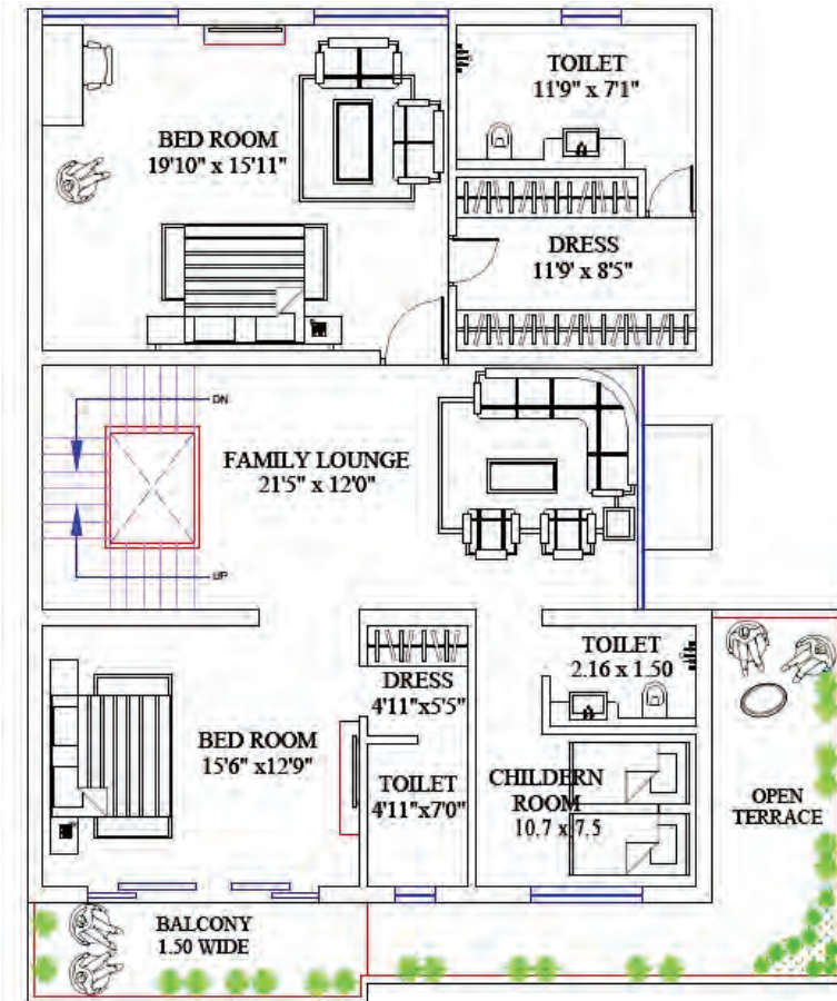
FIRST FLOOR AREA
