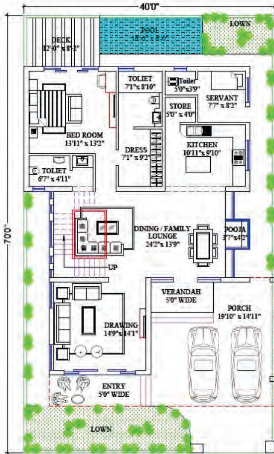
GROUND FLOOR AREA
